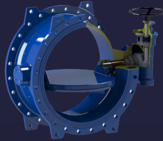
DOUBLE ECCENTRIC BUTTERFLY VALVE
